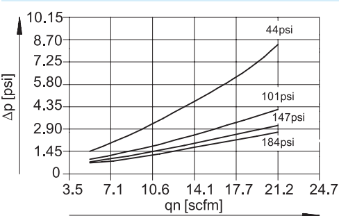
Differential pressure Δp as a function of the standard flow rate at output q n (MS6N-LDM1-...-P30)
