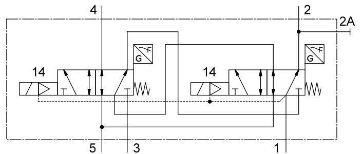
[5L] 5/2-Wegeventil, monostabil
