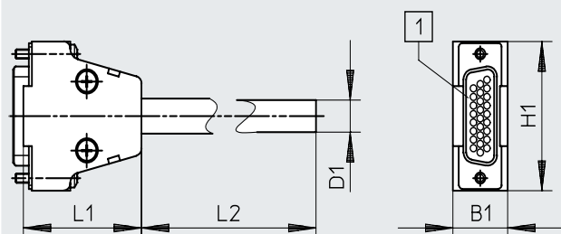
[1] Dose Sub-D, gerade, 26-polig
