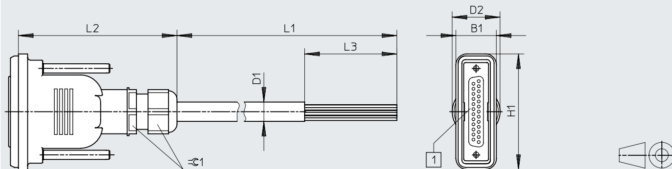
[1] Dose Sub-D, gerade, 44-polig
