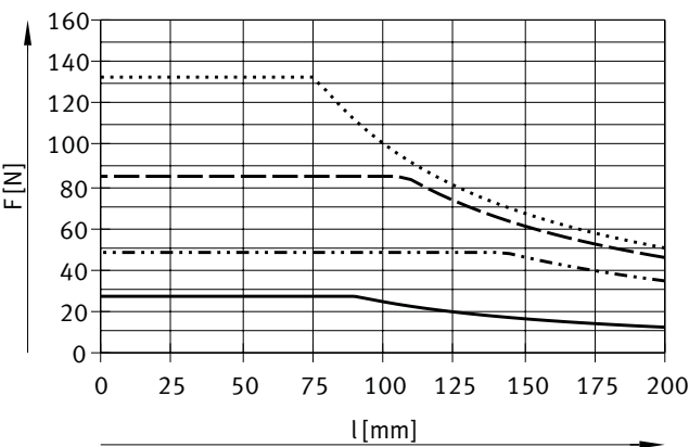
DFM-12 ... 25-KF, Hub 40 ... 100 mm
