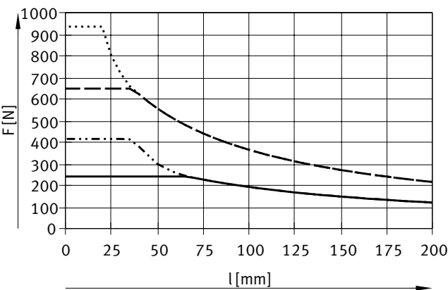
DFM-32 ... 63-KF, Hub 80 ... 100 mm
