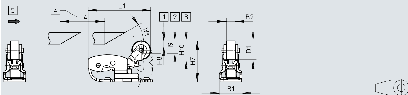
Dimensions – Actuator attachments VAOM, roller lever for 5/2-way valves
