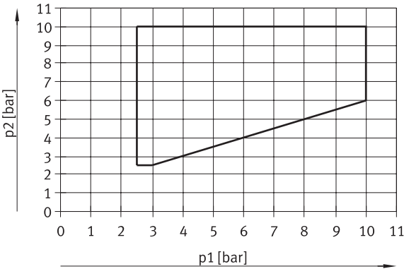
Pilot pressure p2 as a function of external pneumatic spring pressure p1, for piston spool valves VMEF-...-M52...18
