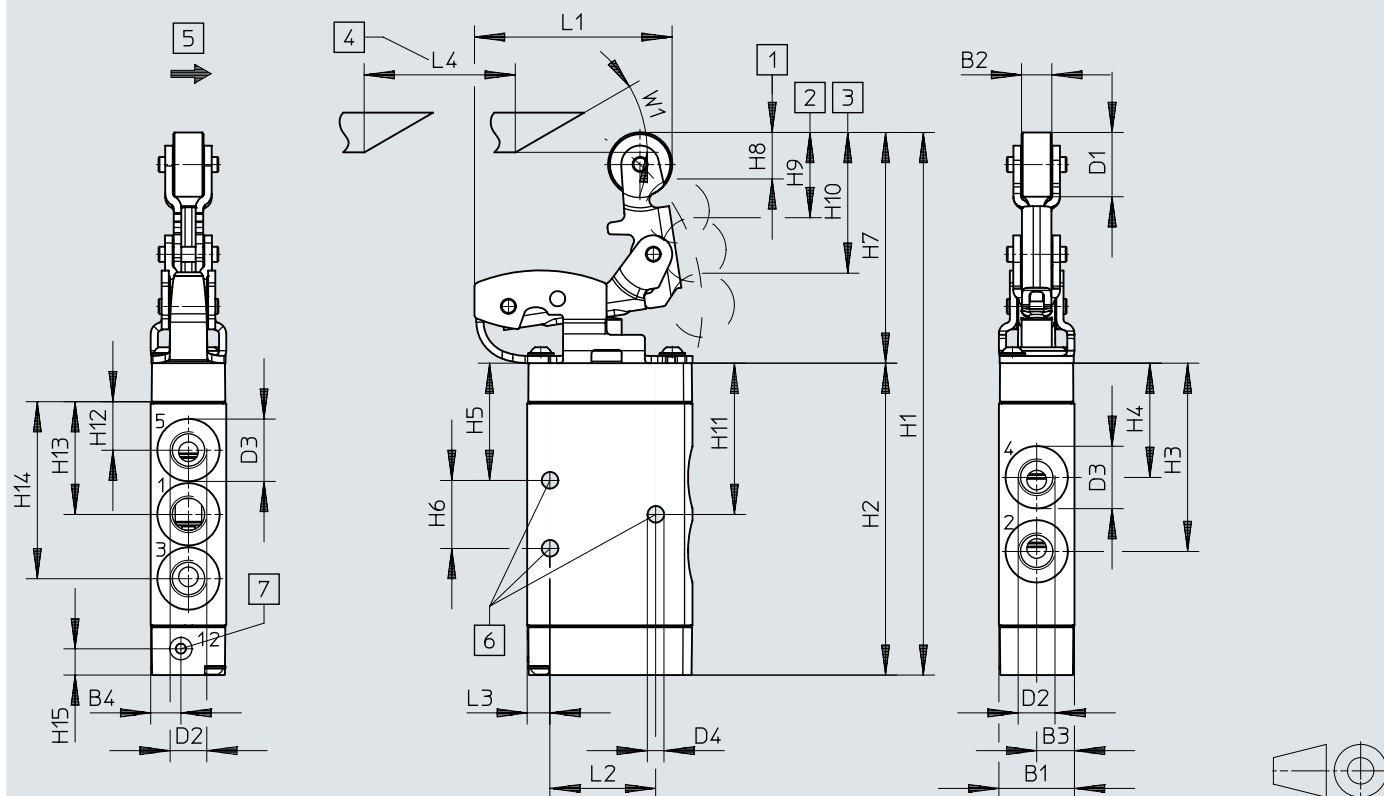
Dimensions – Roller lever valve 5/2-way valve, roller lever with idle return
