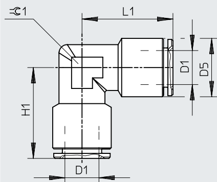
Dimensions – Push-in L-connector NPQM-L
