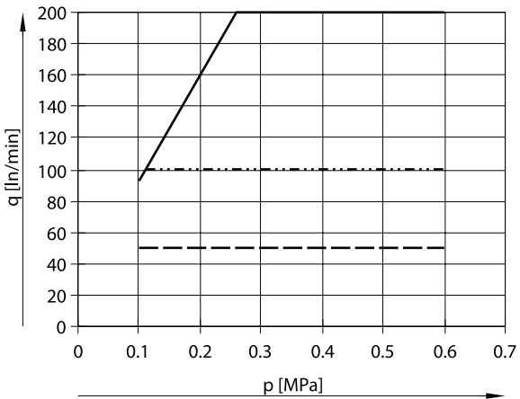
Maximum flow rate in relation to input pressure, at room temperature, nominal width 6 mm, N2
