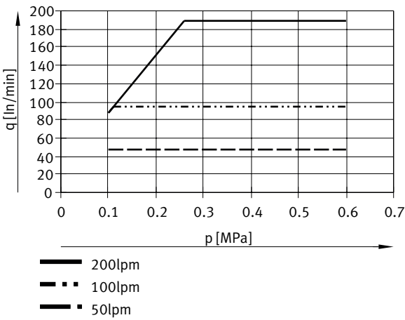
Maximum flow rate in relation to input pressure, at room temperature, nominal width 6 mm, air
