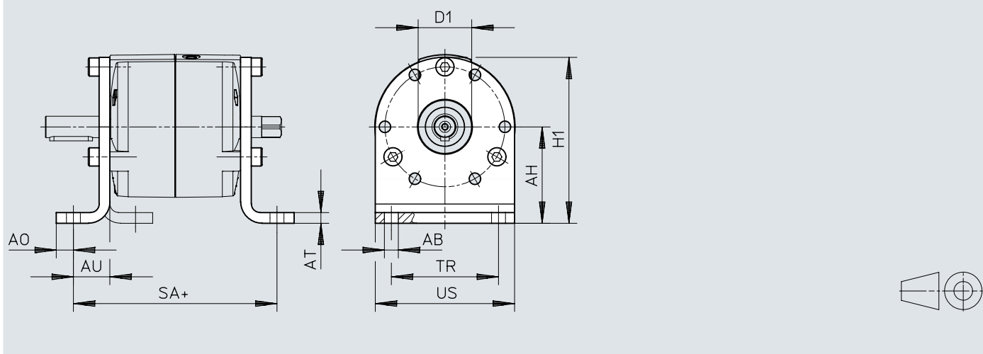
Dimensions – Foot mounting DAMH-Q12-12 ... 25
