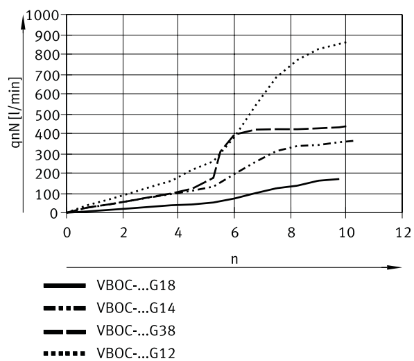
Standard nominal flow q_{nN} at 0.6 → 0.5 MPa as a function of the turns of the adjusting screw n (flow control direction 2 → 1)
