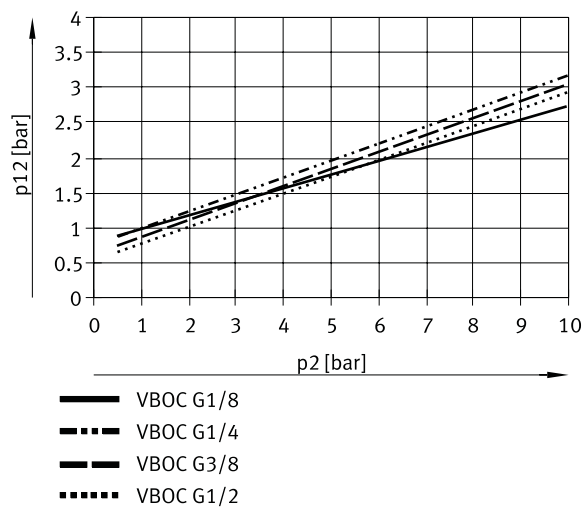
Switch-off pilot pressure p_{12} as a function of operating pressure p_2
