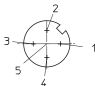
[1] Plug M12x1, 5-pin
