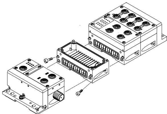
CPX terminal in metal design
