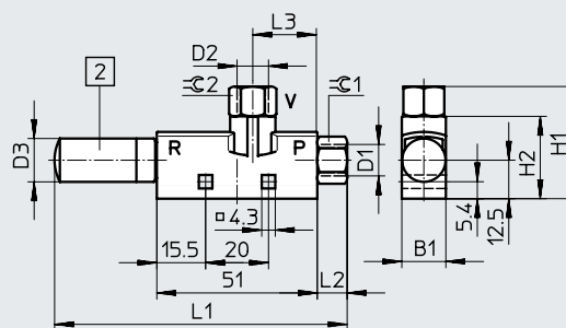
[2] Silencer
