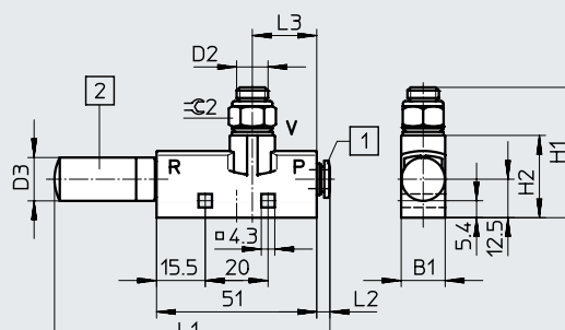
[1] Push-in fitting
