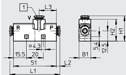
[1] Push-in fitting
