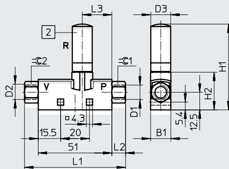
[2] Silencer
