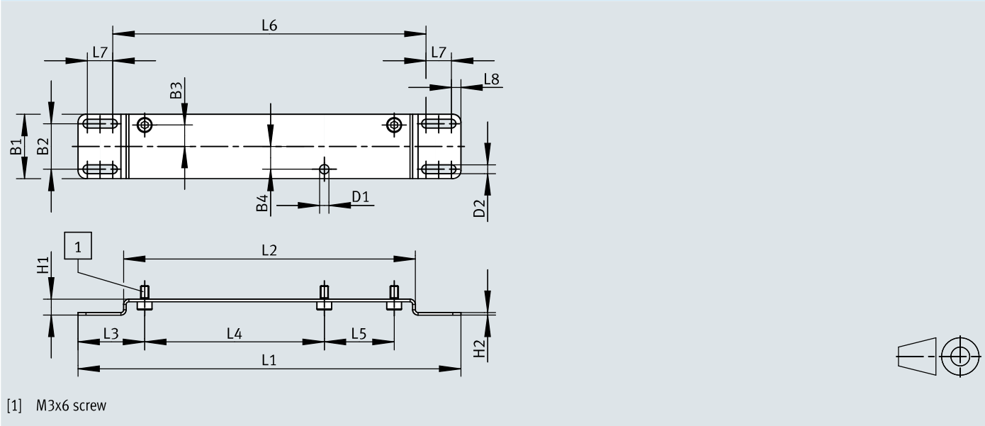
Dimensions – Mounting kit VAME
