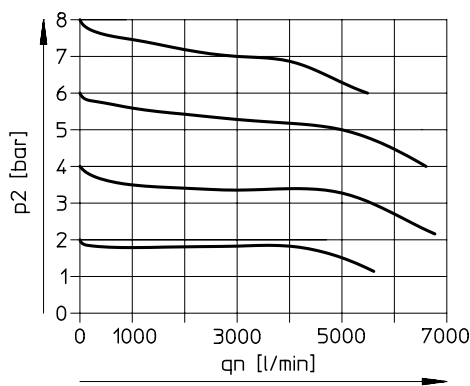
Standard flow rate q_n as a function of output pressure p_2 (combination 1)
