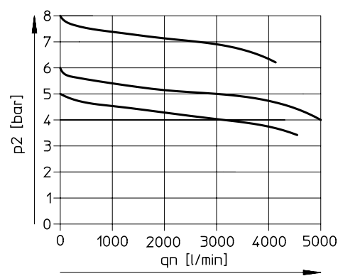
Standard flow rate q_n as a function of output pressure p_2 (Combination 4)
