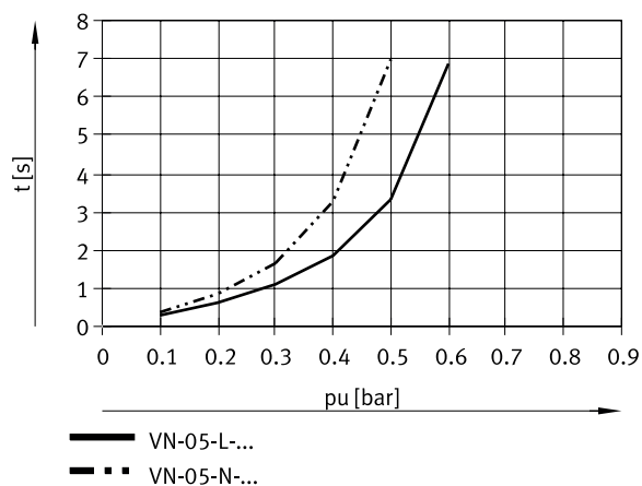
Evacuation time t as a function of vacuum p_u for 1 l volume at 6 bar operating pressure – high suction rate (VN-05-L/N)
