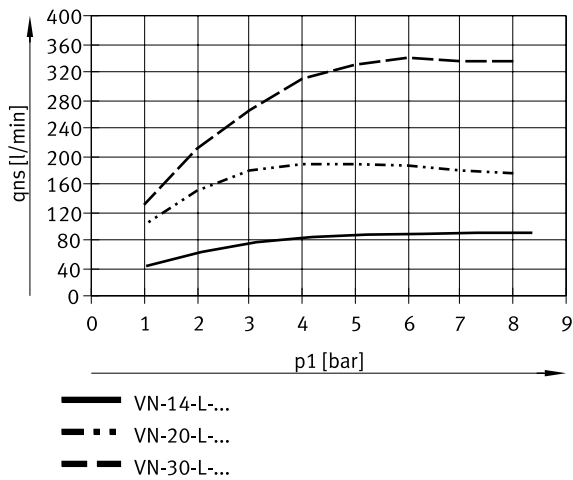
Suction rate q_{ns} (against atmosphere) as a function of operating pressure p_1 – high suction rate (VN-14/20/30-L)
