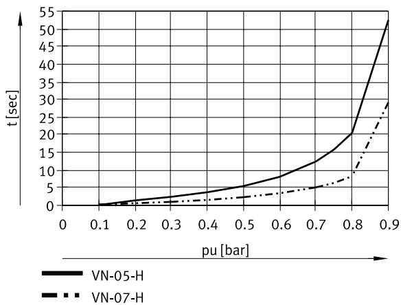
Evacuation time t as a function of vacuum p_u for 1 l volume at 6 bar operating pressure – high vacuum/high suction rate (VN-05/07-H-...-P)
