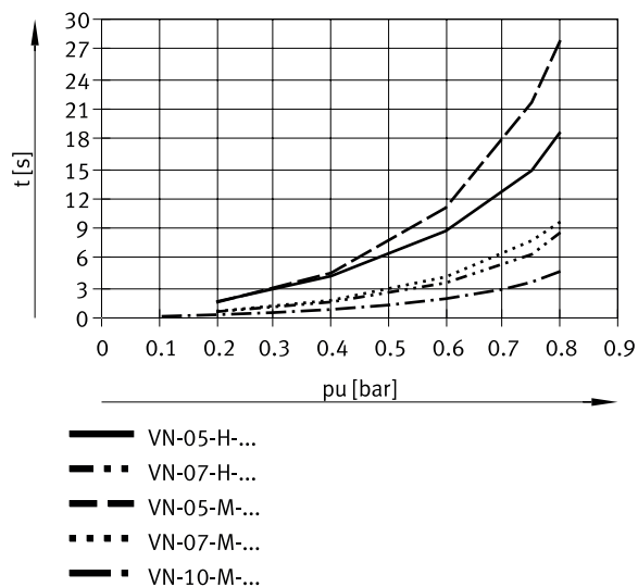
Evacuation time t as a function of vacuum p_u for 1 l volume at 6 bar operating pressure – high vacuum (VN-05/07-H; VN-05/07/10-M)
