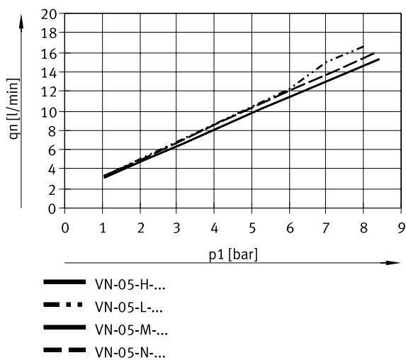
Air consumption q_n as a function of operating pressure p_1 – high vacuum / high suction rate (VN-05-H/L/M/N)
