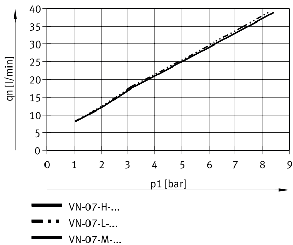
Air consumption q_n as a function of operating pressure p_1 – high vacuum / high suction rate (VN-07-H/L/M)
