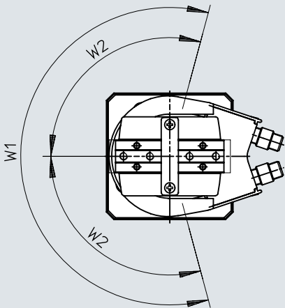
Dimensions – Swivel/gripper units HGDS – swivel angle
