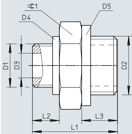
Dimensions – Double nipple NPFC-DS, G thread
