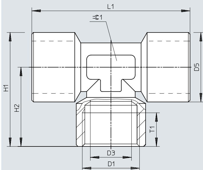
Dimensions – T-fitting NPFC-T, female thread
