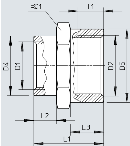
Dimensions – Reducing sleeve NPFC-R
