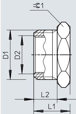
Dimensions – Reducing nipple NPFC-R, male thread/female thread
