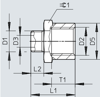
Dimensions – Reducing nipple NPFC-R, female thread/male thread
