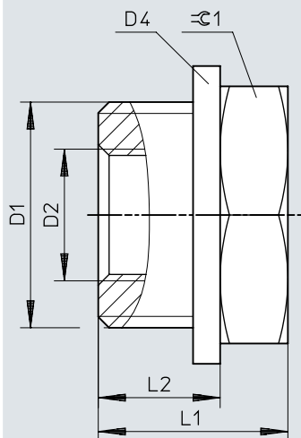
Dimensions – Reducing nipple NPFC-RS, G thread
