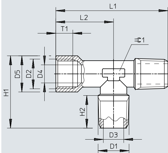
Dimensions – T-fitting NPFC-T, male thread/male thread/female thread
