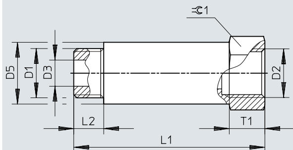
Dimensions – Extension NPFC-E...
