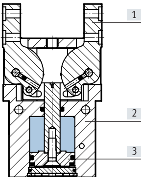
Radial gripper
