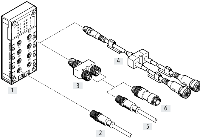
Combination of connection block and electrical connection technology
