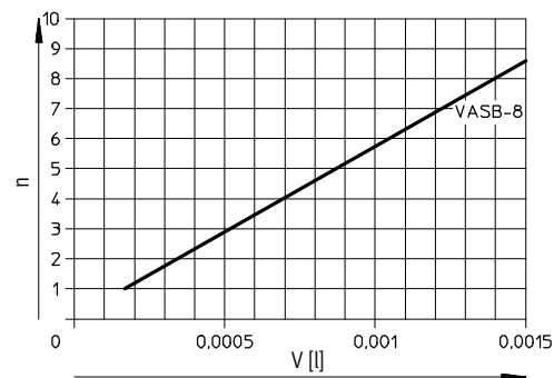
Suction cup volume
