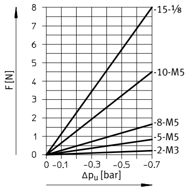
Theoretical suction force F as a function of vacuum p_u
