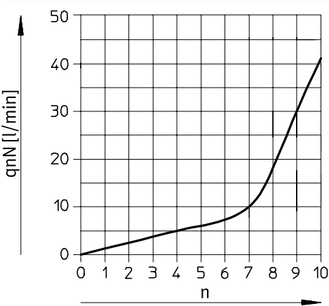
Standard nominal flow rate q_{nN} at 6 → 5 bar as a function of spindle rotations n
