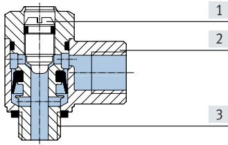
One-way flow control valve
