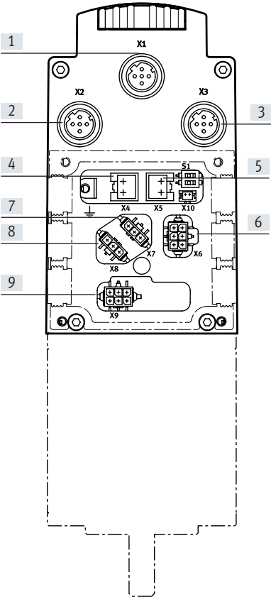
EMCA-...-PN/-EP/-EC
