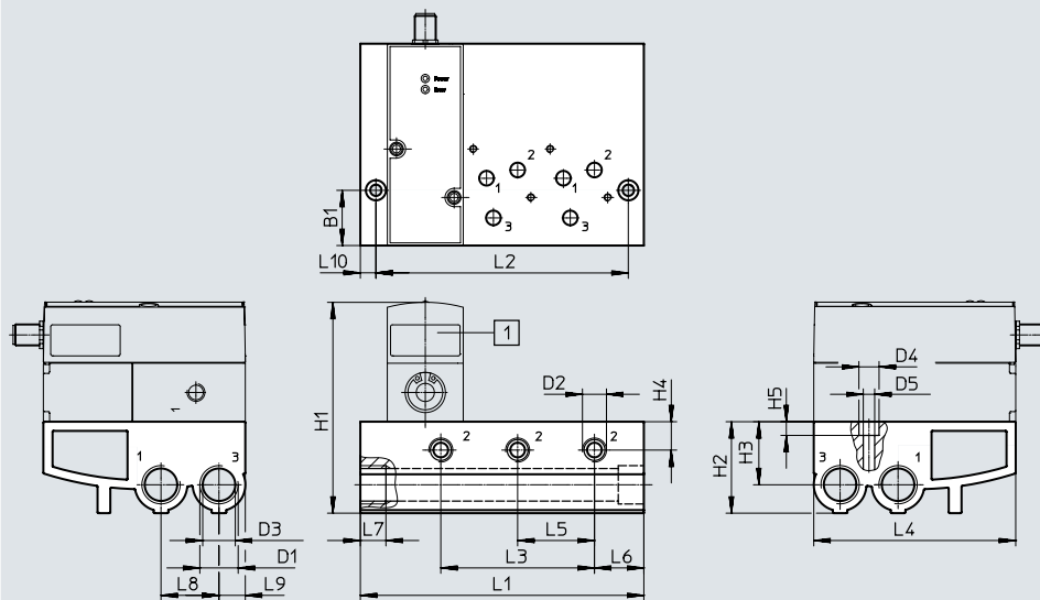
[1] Proportional pressure regulator VPPX
