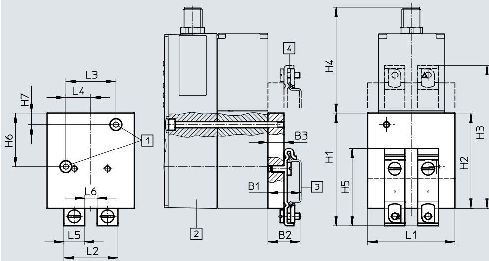
[1] Socket head screw M4 [2] Proportional-pressure regulator VPPX [3] H-rail NRH [4] H-rail mounting can be rotated by 180° if required
