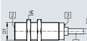
M18 – Flush fitting Cable
