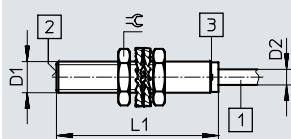
M12 – Flush fitting Cable
