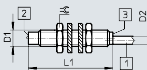
M12 – Partially flush fitting Cable
