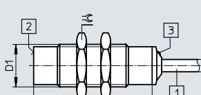
M18 – Partially flush fitting Cable
