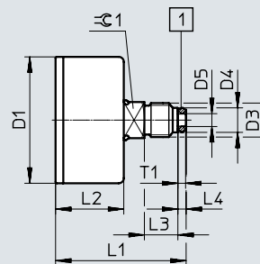
MA-50, G1/4
