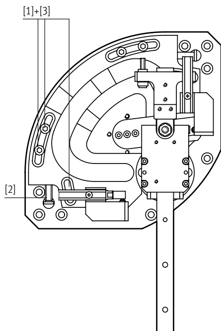
Swivel angle
