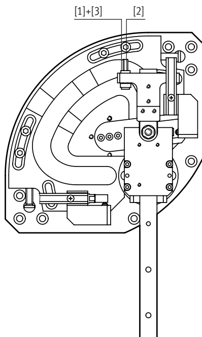
Linear stroke
