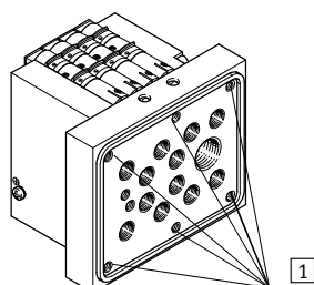
1 Mounting holes
