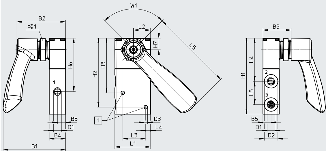
[1] Mounting holes for screws M4
