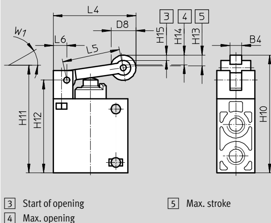
Roller lever valve R-3-1/4-B, R0-3-1/4-B
