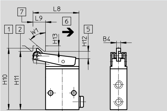
Toggle lever valve LS-3-1/8, LOS-3-1/8
