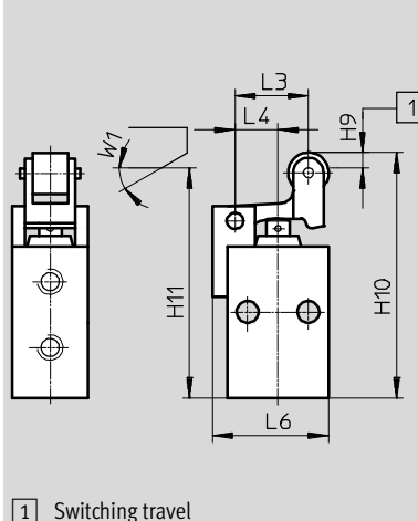
Roller lever valve R-3-M5
