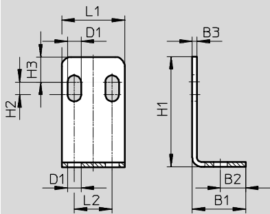
Mounting bracket HV-M5
