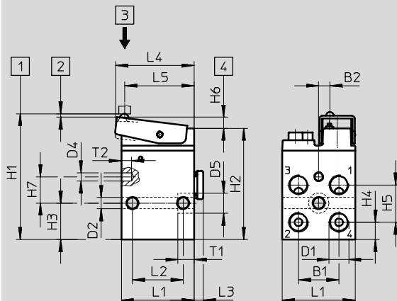
Stem actuated valve VS-4-1/8
