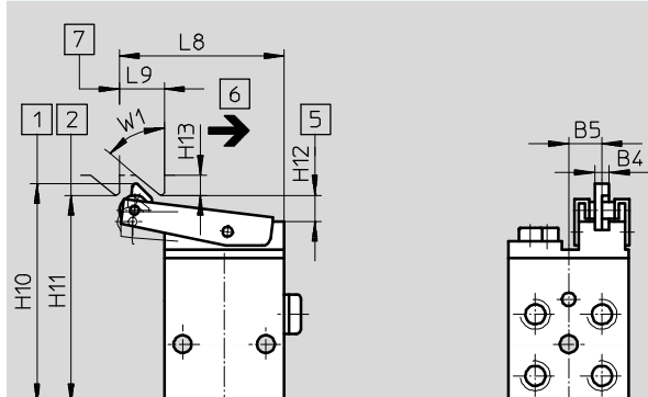
Toggle lever valve LS-4-1/8
