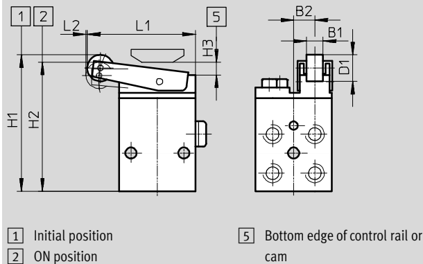
Roller lever valve RS-4-1/8
