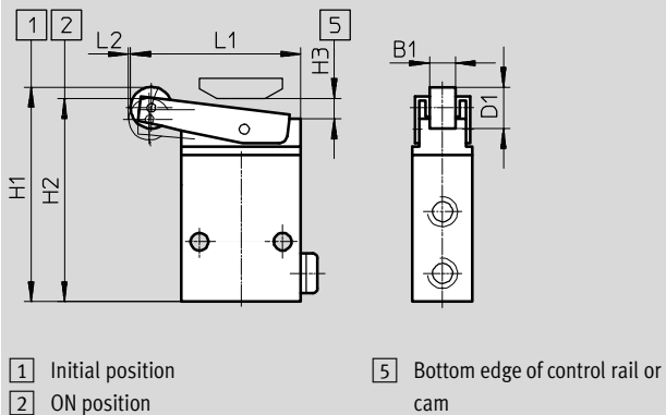
Roller lever valve RS-3-1/8, ROS-3-1/8
