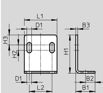
Mounting bracket HV-1/8
