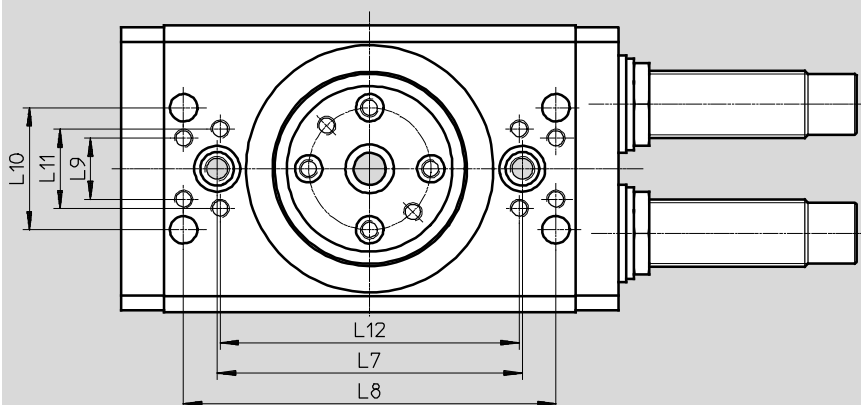
DRRD-32 ... 40
