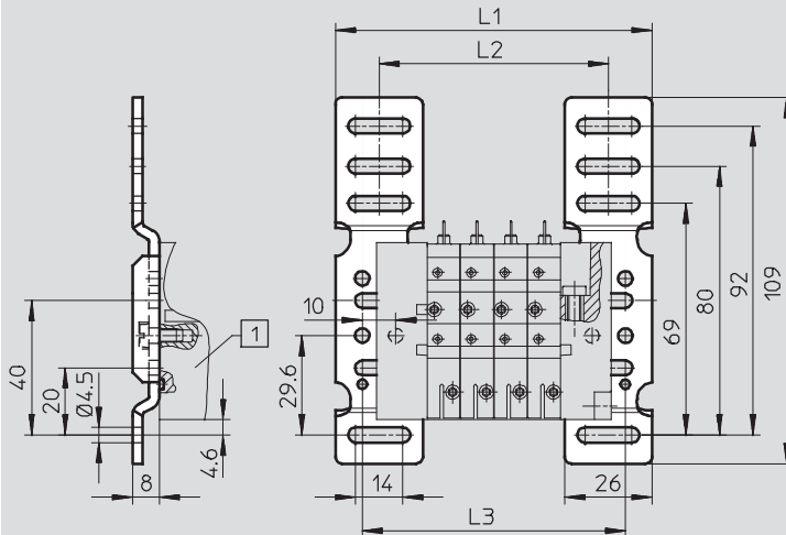
1 Valve terminal CPV-...
