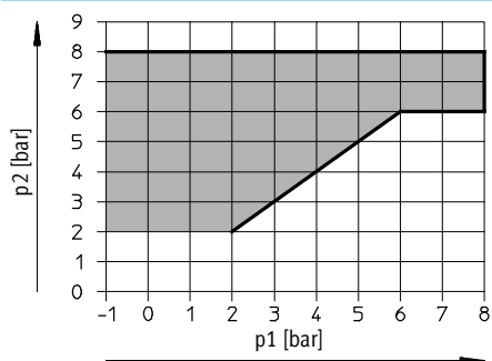
Pilot pressure p2 as a function of working pressure p1
