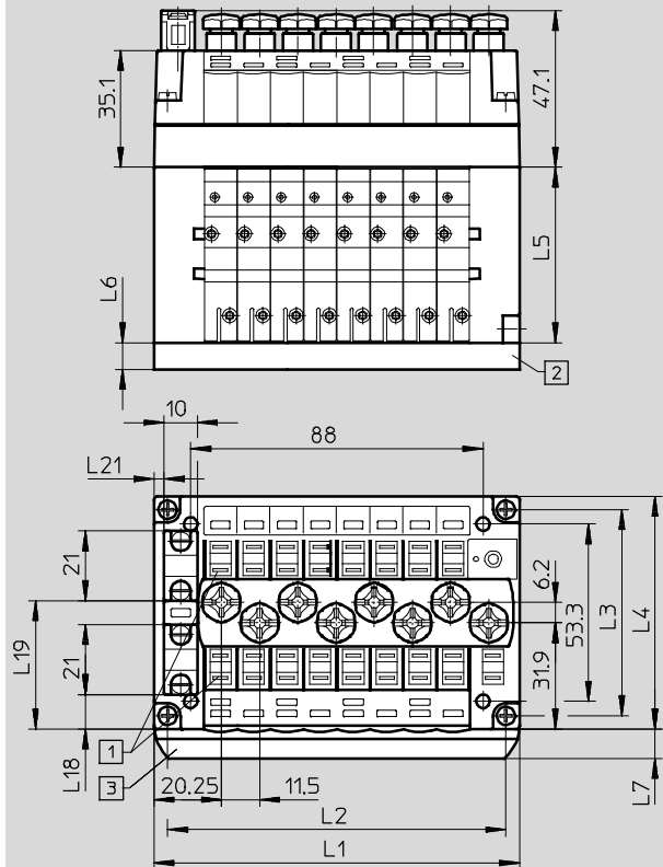
Valve terminal with AS-interface connection and additional inputs – CPV10
