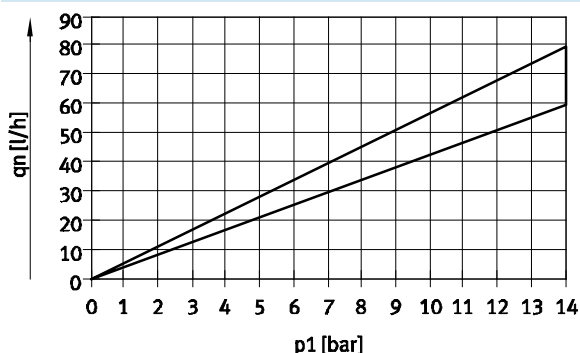
Internal air consumption q_n as a function of input pressure p_1
