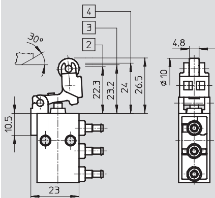
Roller lever valve with idle return L/O
