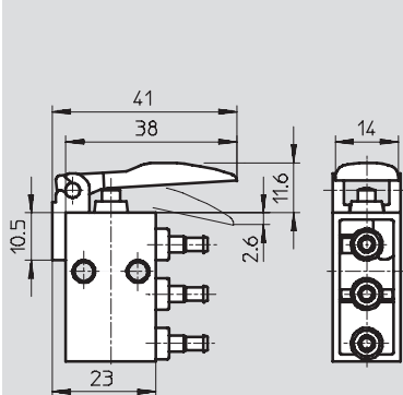
Finger lever valve TH/O
