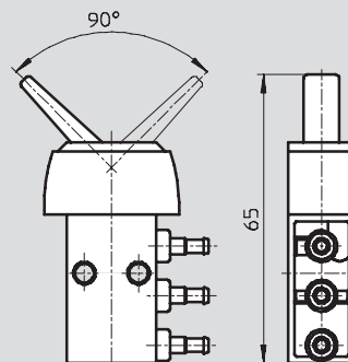
Toggle lever valve KH/O
