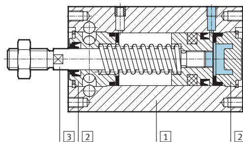
Sectional view EMM(L) – Pushing
