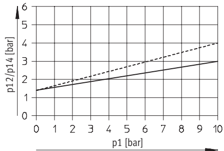
MVH-5-1/8-S-B
