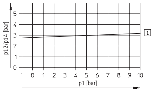
MFH-5/3...-3/8-S-B
