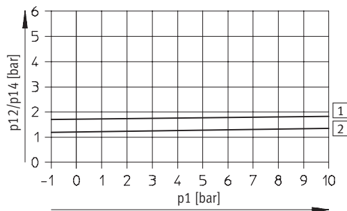
MVH-5-3/8-S-B
