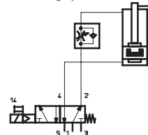
Actuating cylinder
