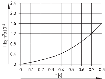
Opening and closing times t as a function of gripper finger mass moment of inertia J
