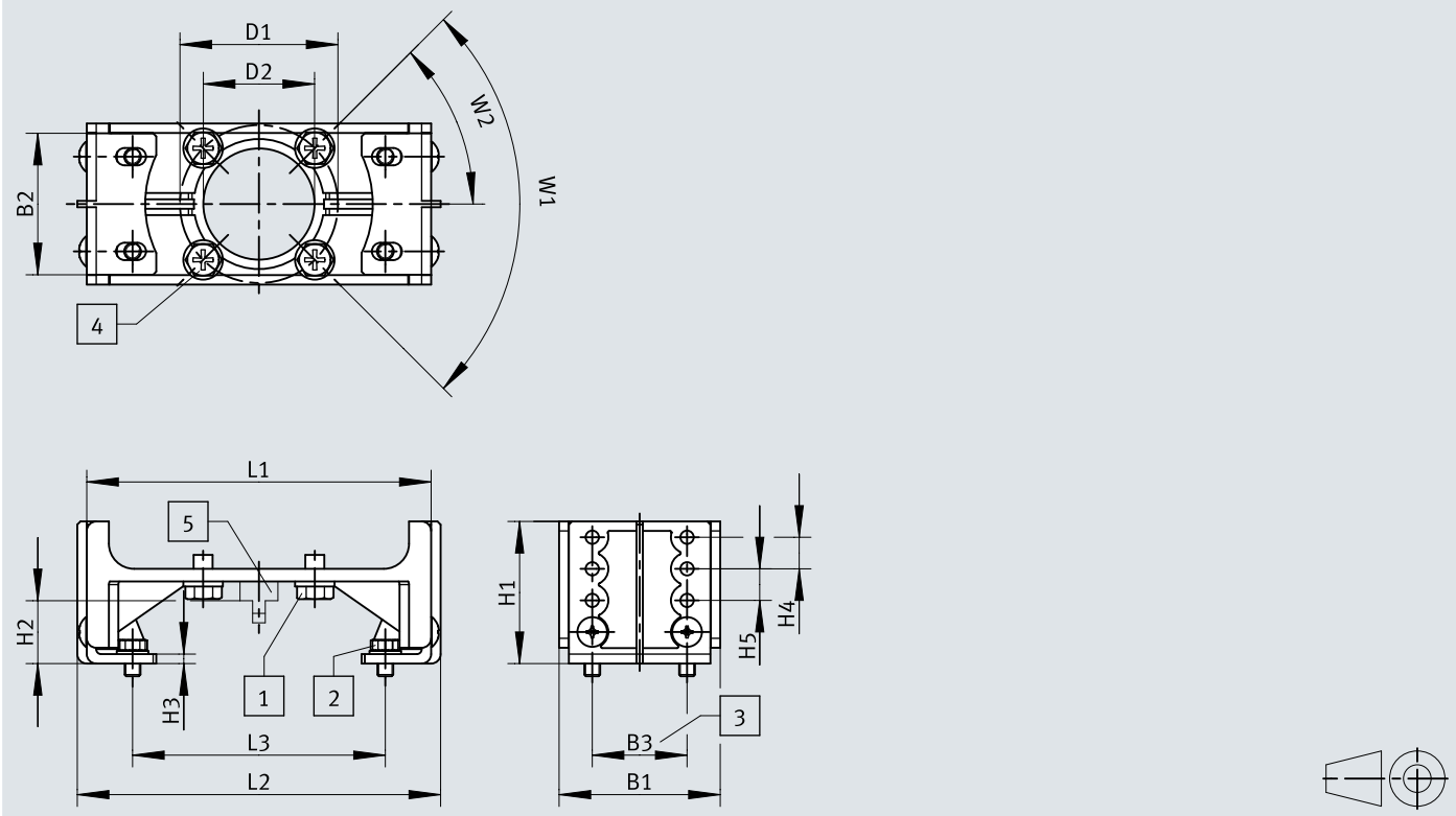
Dimensions – Mounting adapter DARQ with mounting brackets fitted facing inwards
