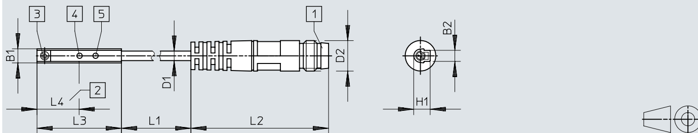
Dimensions – SME-10 plug, connection outlet direction lengthways
