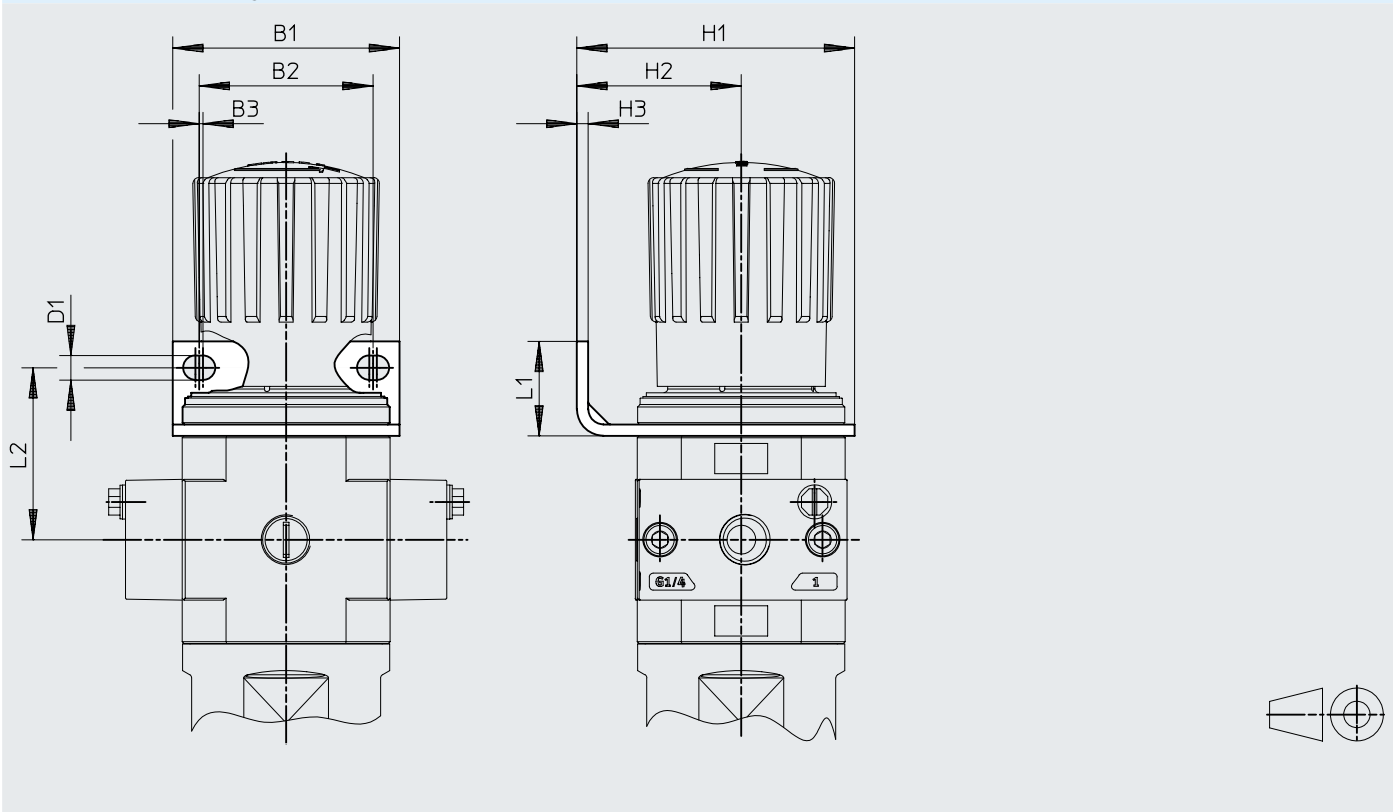
Dimensions – With mounting bracket HR-D-R3
