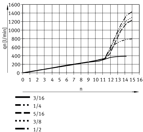
Standard flow rate q_n at 6 → 0 bar depending on the turns of the flow control screw n (pneumatic connection NPT3/8-18)
