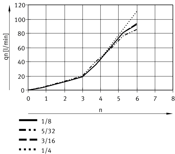
Standard flow rate q_N at 6 \rightarrow 0 bar depending on the turns of the flow control screw n (pneumatic connection UNF10-32)
