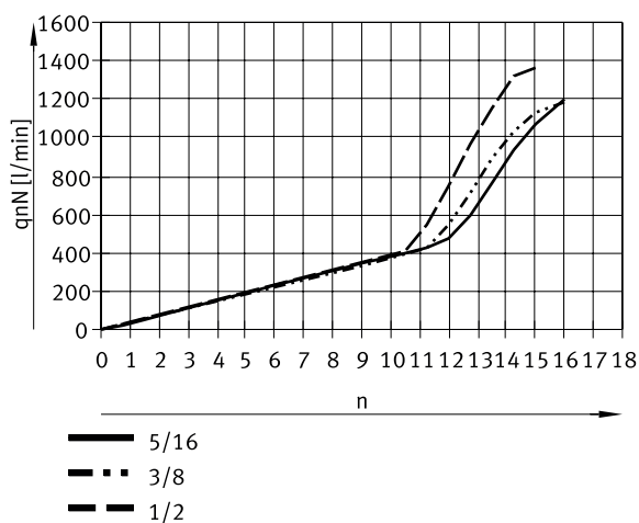
Standard nominal flow rate q_n at 6 bar → 0 bar depending on the adjusting screw n (GRLA-1/2-QB-...-U)
