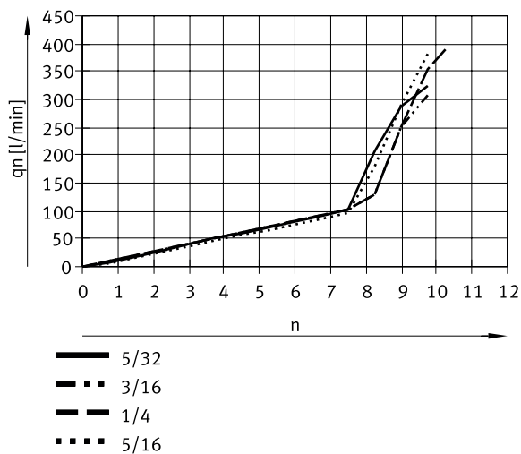
Standard flow rate q_n at 6 → 0 bar depending on the turns of the flow control screw n (pneumatic connection NPT1/8-27)
