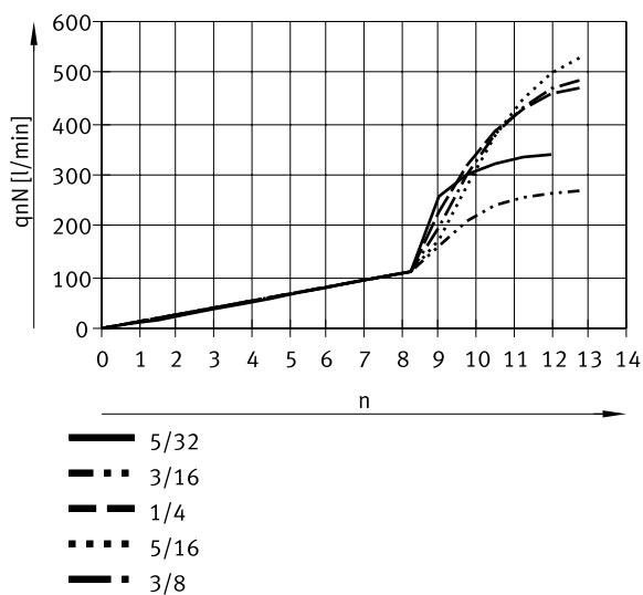
Standard nominal flow rate q_n at 6 bar → 0 bar depending on the adjusting screw n (GRLA-1/4-QB-...-U)
