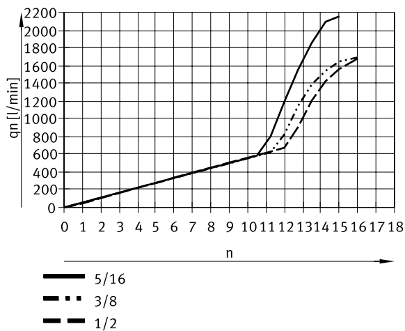
Standard flow rate q_n at 6 → 0 bar depending on the turns of the flow control screw n (pneumatic connection NPT1/2-14)
