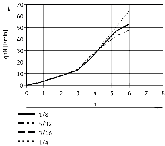
Standard nominal flow rate q_N at 6 bar \rightarrow 0 bar depending on the adjusting screw n (GRLA-10-32UNF-QB-...-U)
