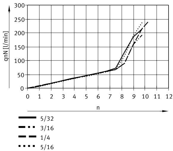
Standard nominal flow rate q_N at 6 bar \rightarrow 0 bar depending on the adjusting screw n (GRLA-1/8-QB-...-U)
