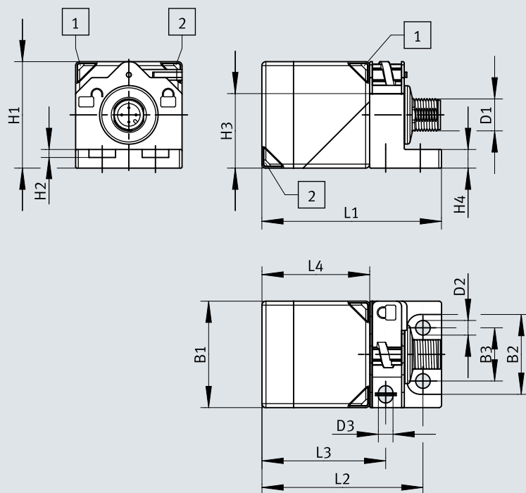
Dimensions – SOIA-Q40NB-PNLK-M12
