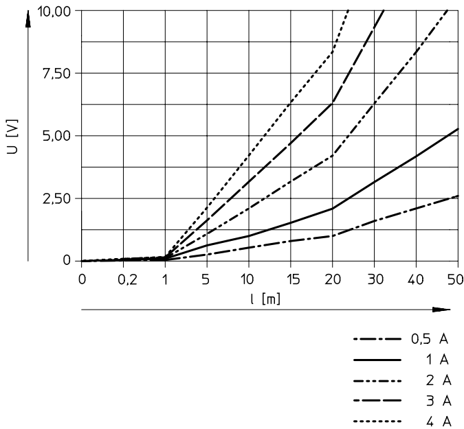
Voltage drop U for cable cross-section 0.34 mm 2 with M12
