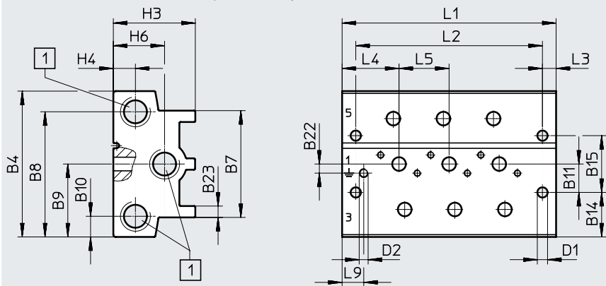
[1] Port 1, 3 and 5: G1/4
