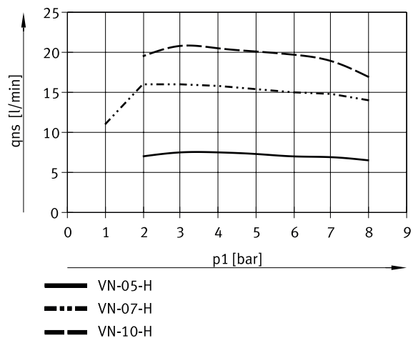
Suction rate q_{ns} (against atmosphere) as a function of operating pressure p_1 – high vacuum (VN-05/07/10)
