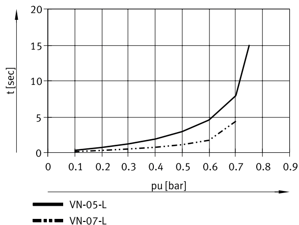
Evacuation time t as a function of vacuum p_u for 1 l volume at 6 bar operating pressure – high suction rate (VN-05/07)
