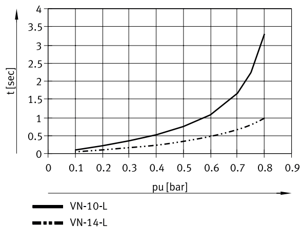
Evacuation time t as a function of vacuum p_u for 1 l volume at 6 bar operating pressure – high suction rate (VN-10/14)
