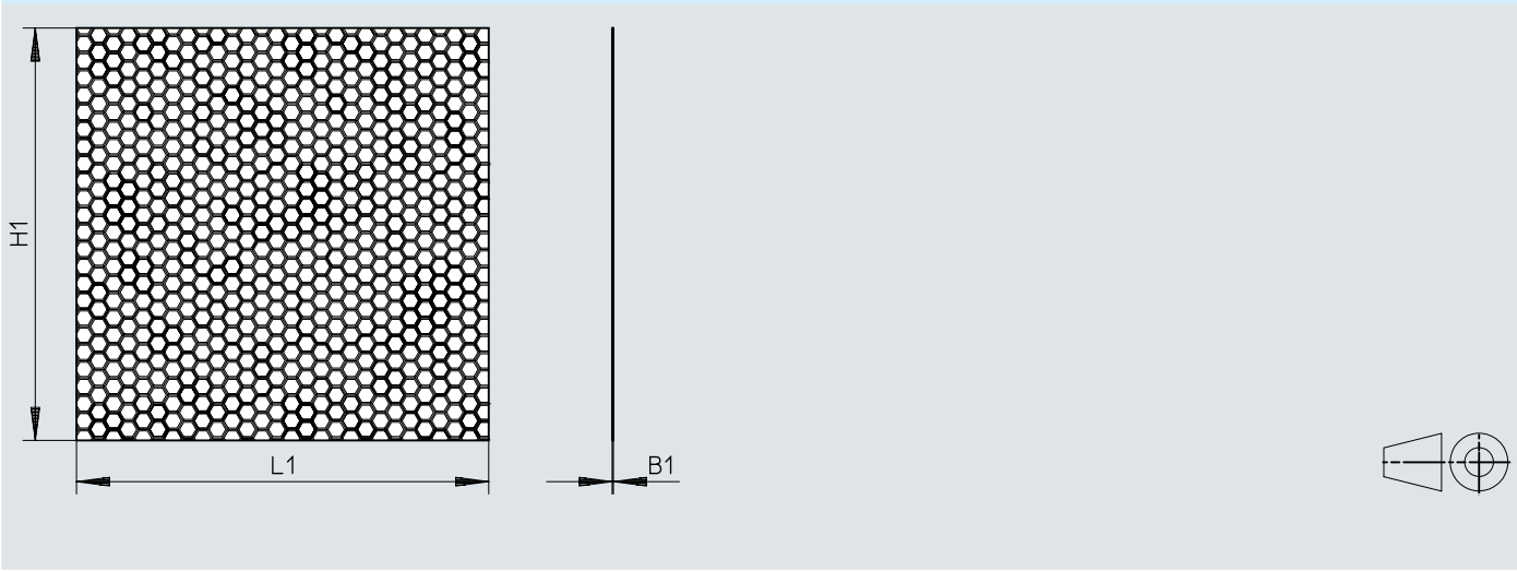
Dimensions – Reflector foil SARA-RF-Q100
