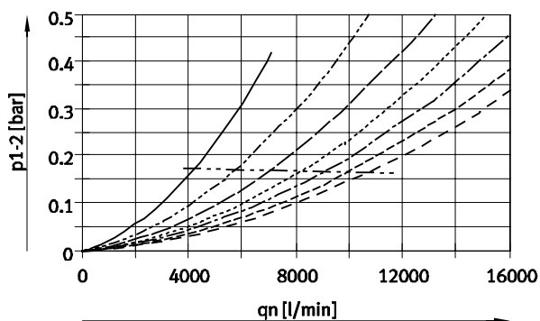
Standard flow rate q_n as a function of differential pressure \Delta p_{1-2} (pneumatic connection 3/4 NPT – high flow rate HF)
