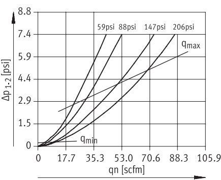
Standard flow rate q_n as a function of differential pressure \Delta p_{1-2} (MS6N-LFM-1/4)
