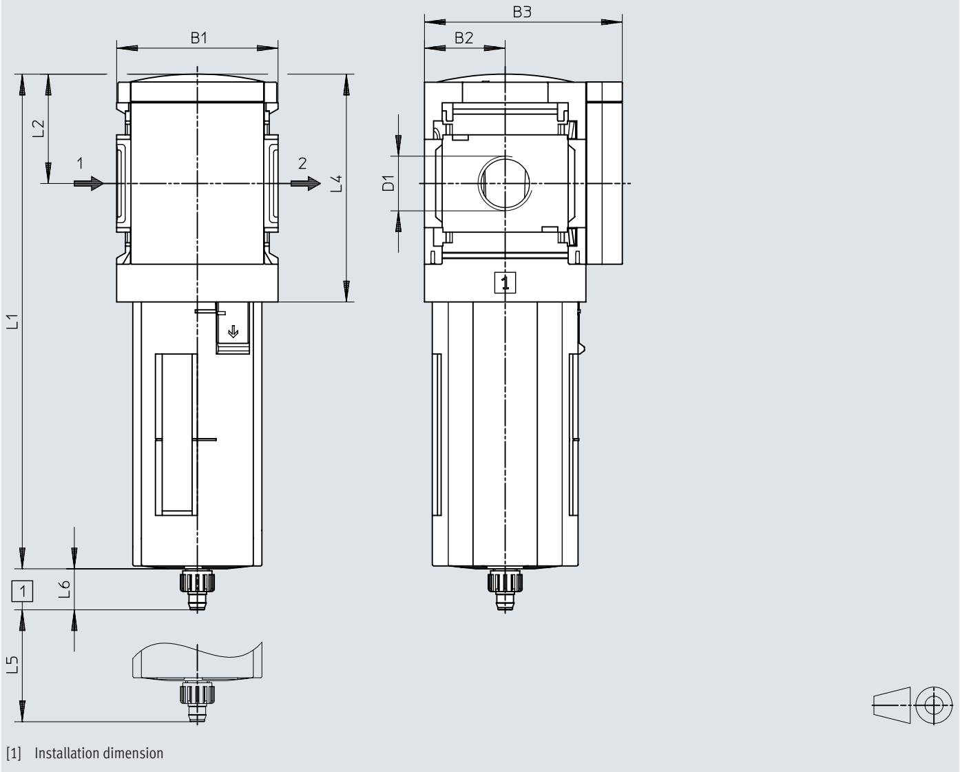
Dimensions – Condensate drain, manual, rotary, with plastic bowl guard R
