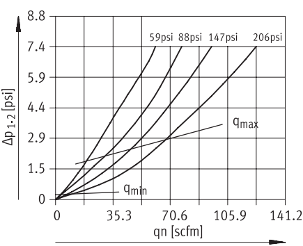
Standard flow rate q_n as a function of differential pressure \Delta p_{1-2} (MS6N-LFM-3/8)
