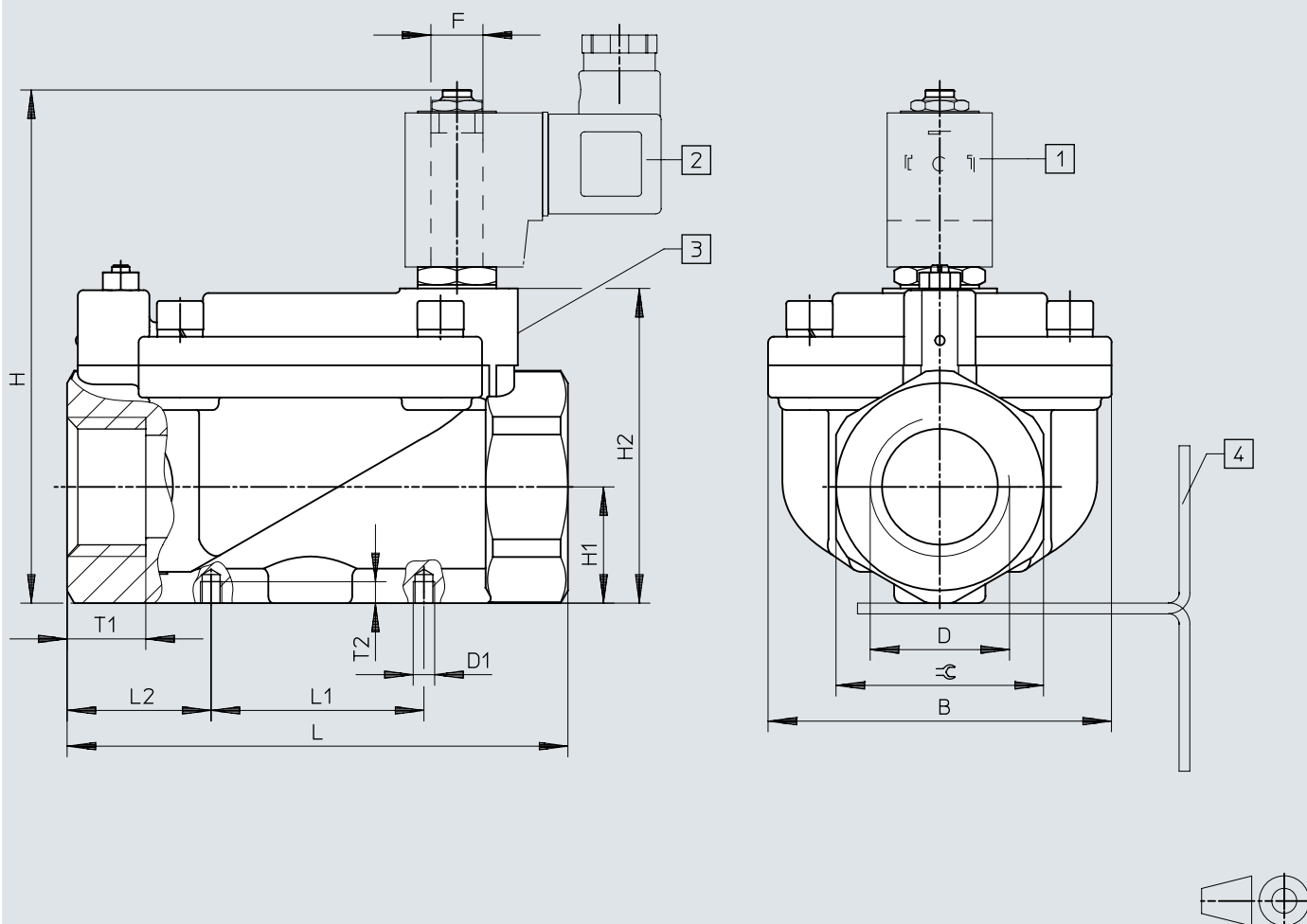
Dimensions – 2/2-way valve, NPT
